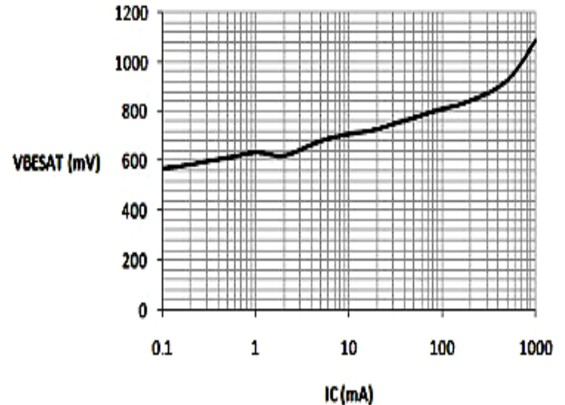
Fig 5: Base Emitter Saturation Voltage vs Collector Current
