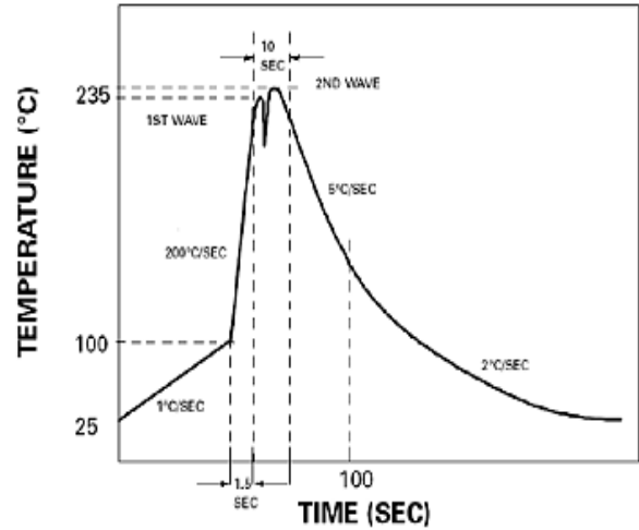
The Recommended solder Profile For Devices
