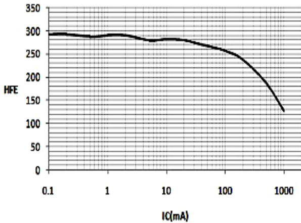
Fig 1: DC Current Gain vs Collector Current
