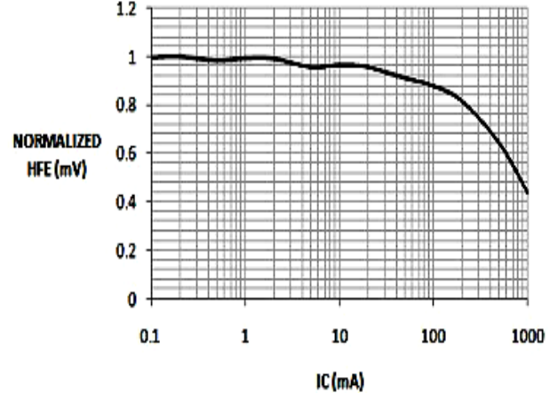
Fig 4: Normalized hFE vs Collector Current
