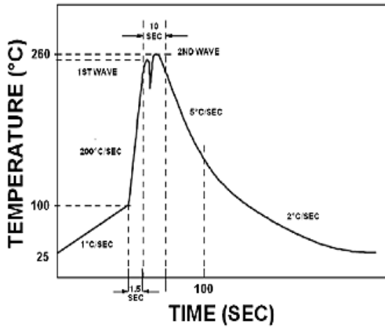
The Recommended solder Profile For Devices
